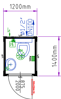
Conteneur WC 5'
