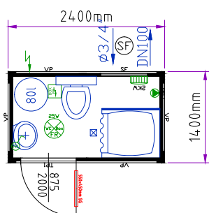
Conteneur WC-douche 8'
